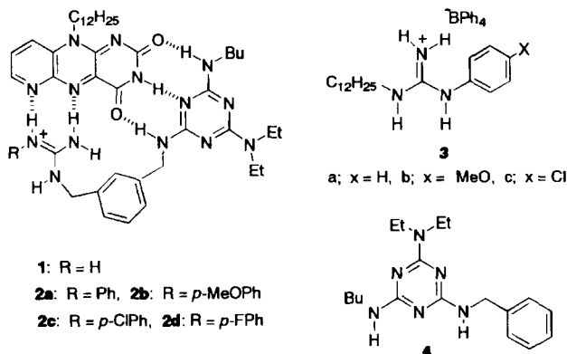
Chart 1. Complex of 6-azaflavin with 1 or 2 and related compounds.
